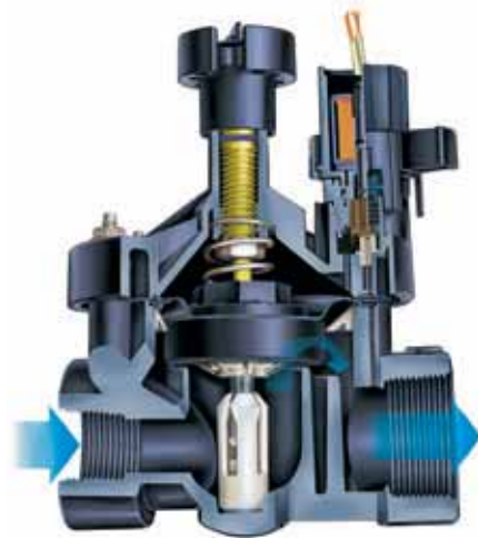
PESB Cutaway
